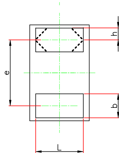
BOTTOM VIEW
